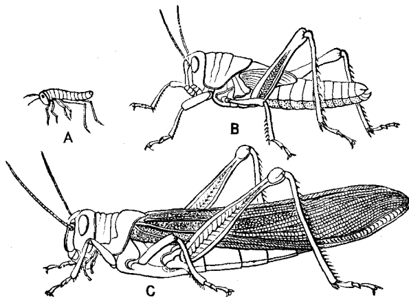
Acridium peregrinum : A, larva, newly hatched; B, pupa, just before its last moult; C, perfect insect.
